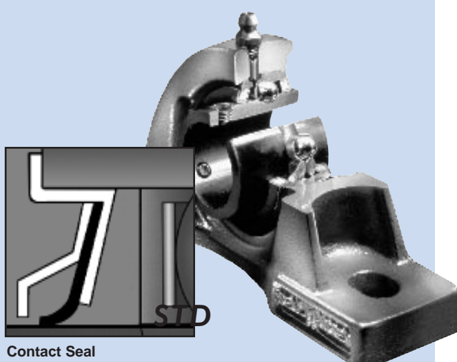
Contact Seal
