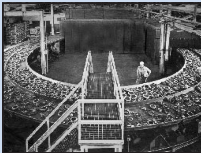
Quality-made SEALMASTER bearings help vibrate 60-tons of conveyor and hot castings in this tough installation. This 45-ton dynamically-balanced conveyor, vibrating at 360 cycles/minute, handles and cools 15 tons of hot foundry castings on a continuous basis. It operates on custom-modified SEALMASTER ball and roller bearings which have special tight housing fit-ups for this demanding vibratory service.
